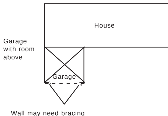
Figure 31—Additional bracing. Home configuration where there is no in-line wall. Additional bracing may be appropriate in this situation.
